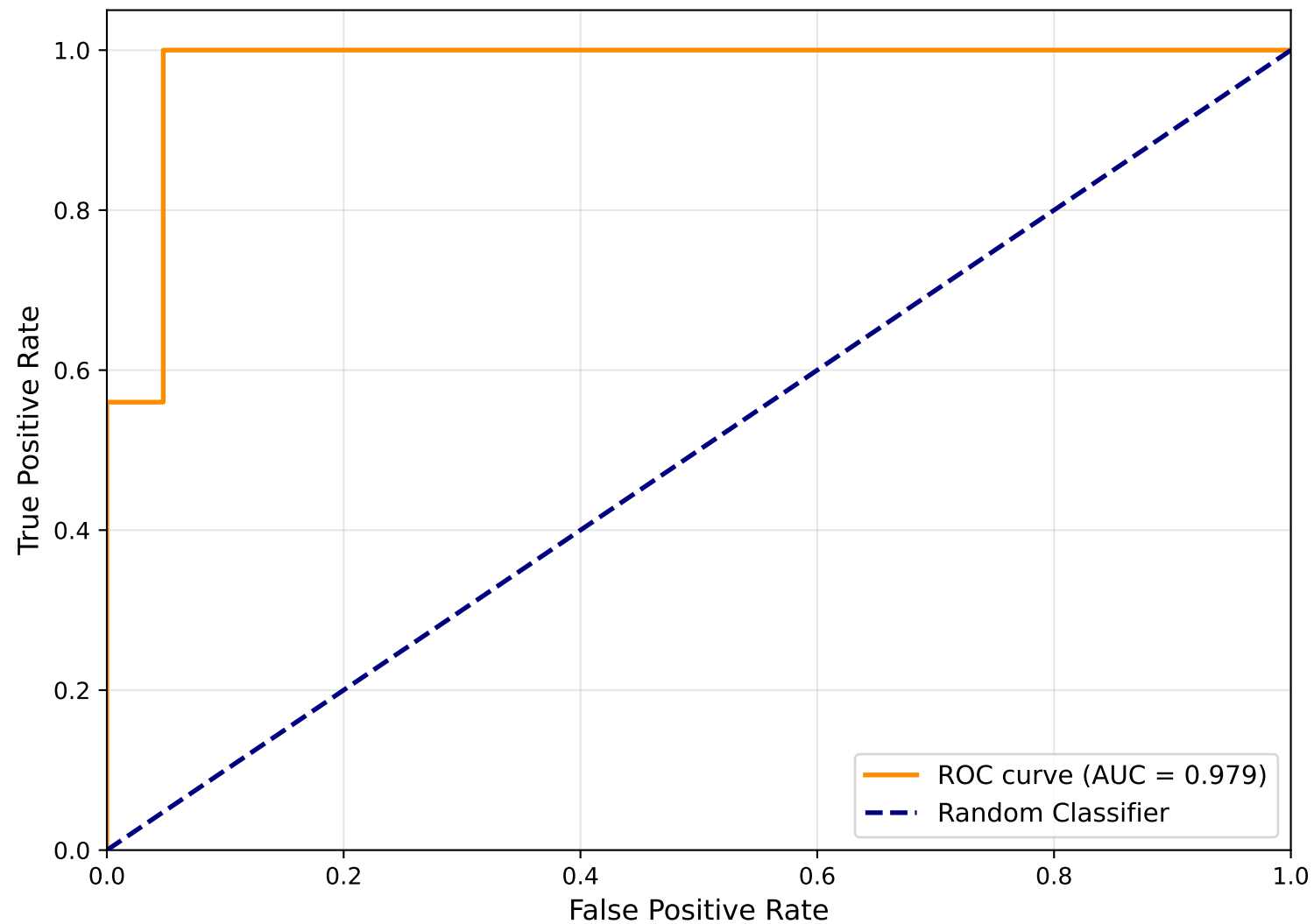
ROC Curve for Tuned CatBoost
